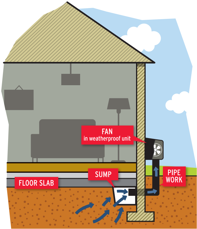
ACTIVE SUMP with fan added and outlet at ground level
